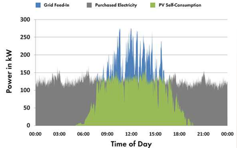
SMA Self Consumption Diagram
